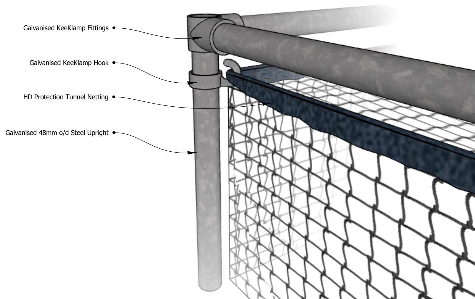
TOP CORNER NETTING DETAIL
