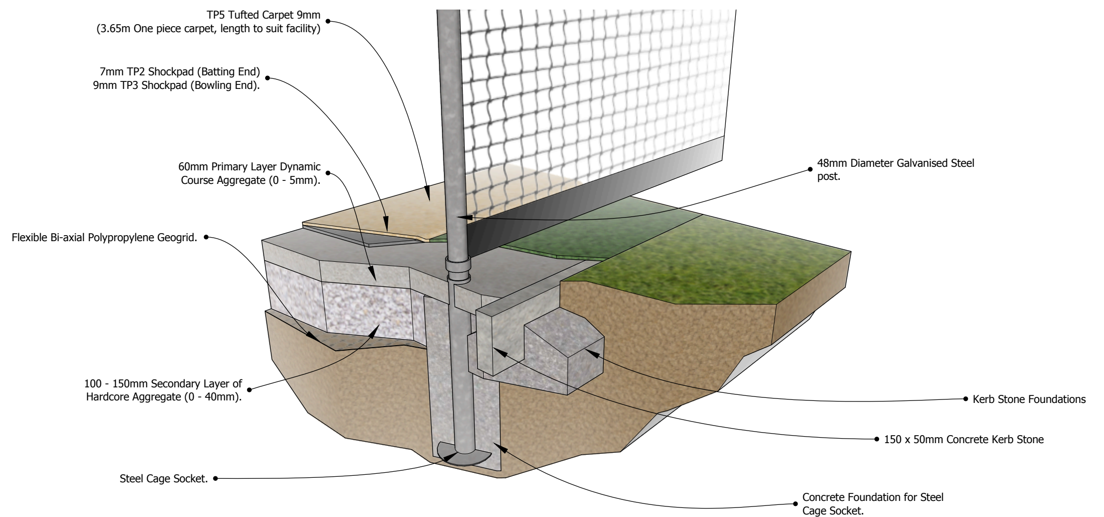
CAGE POST INSTALLATION
