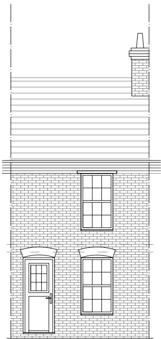
Front Elevation
