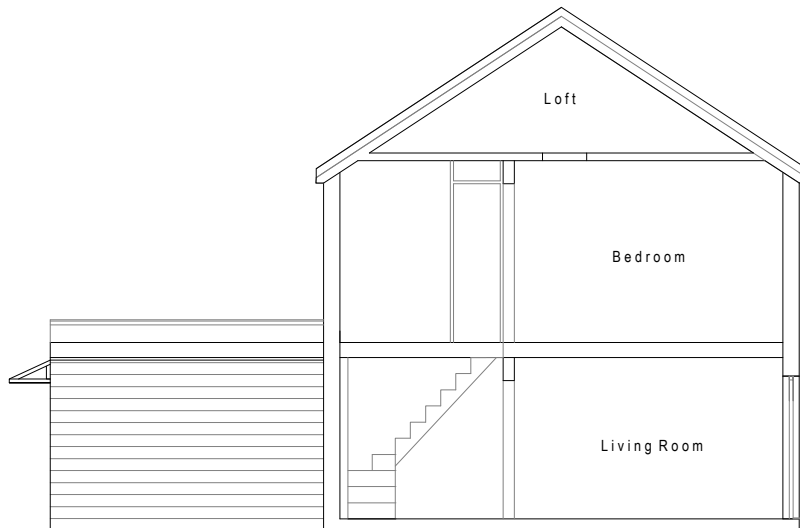
Side Sectional Elevation
