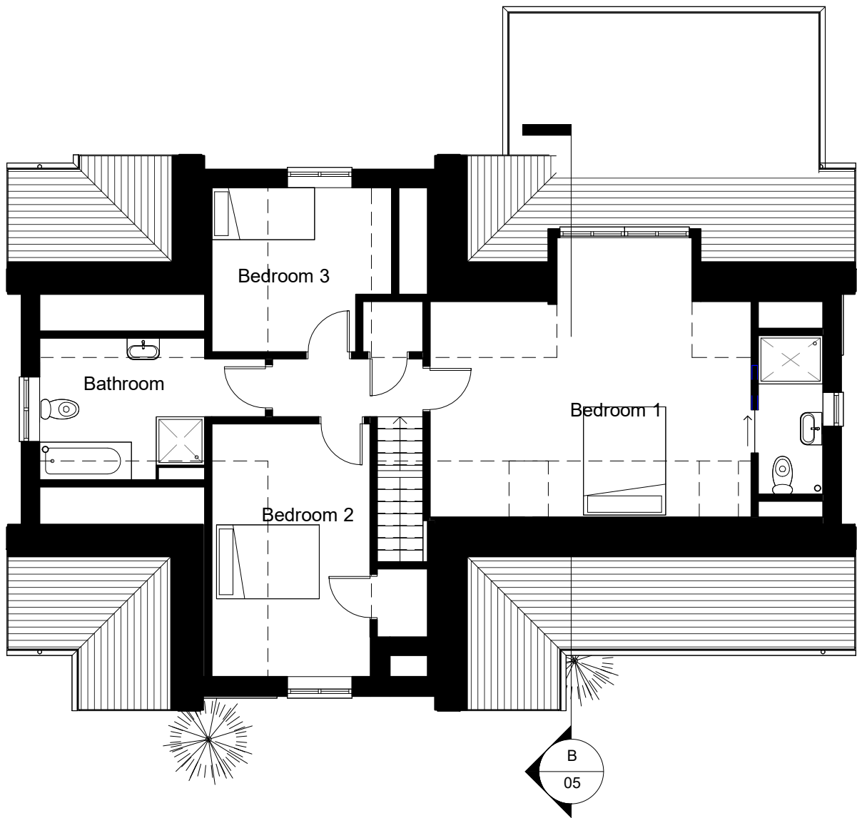
Proposed First Floor 1 : 100
