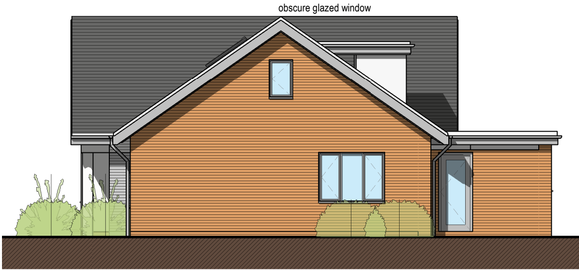
Proposed NorthWest Elevation 1 : 100
