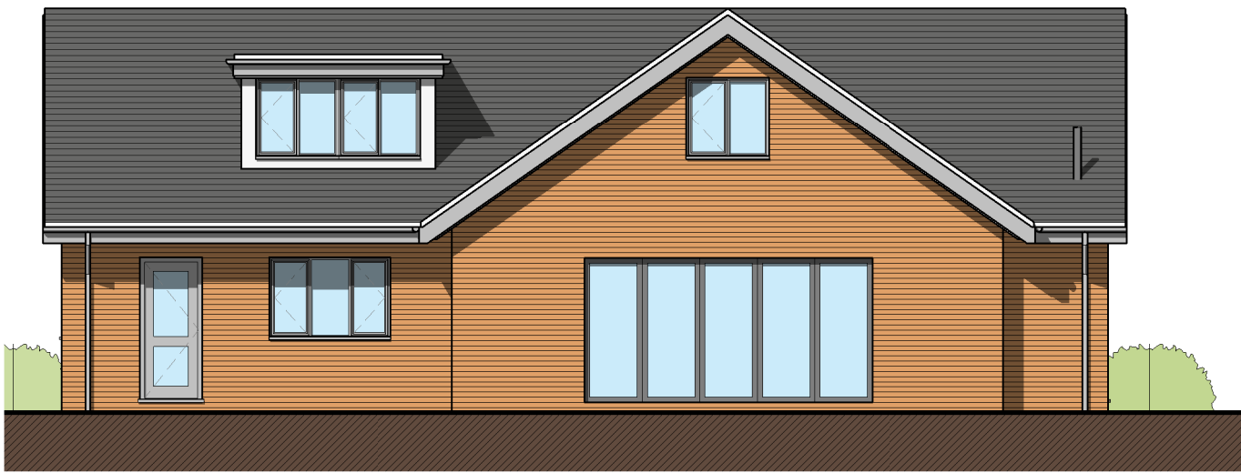
Proposed SouthWest Elevation 1 : 100
