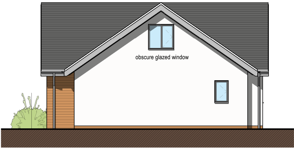
Proposed NorthEast Elevation 1 : 100
