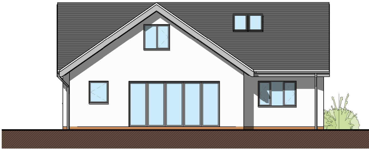
Proposed NorthWest Elevation 1 : 100
