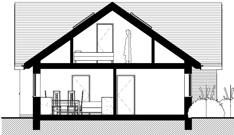
Proposed Section A-A 1 : 100
