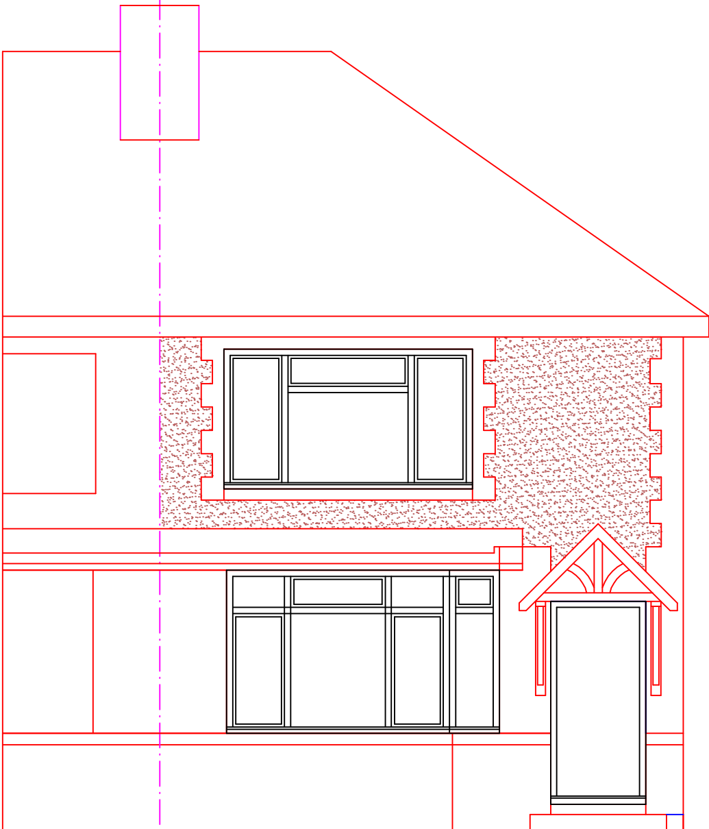
FRONT (STREET) ELEVATION
