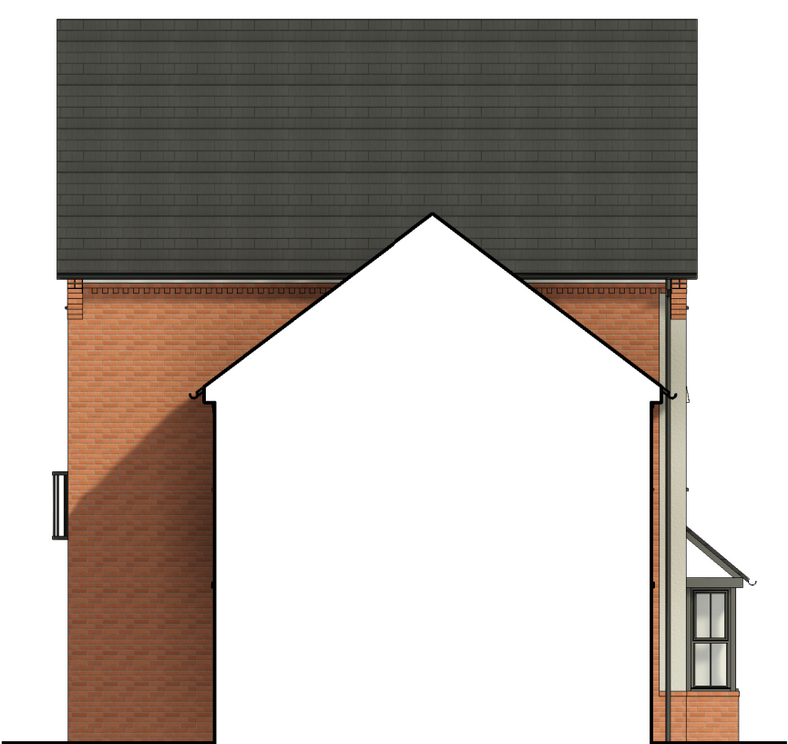
Left Elevation/Section
