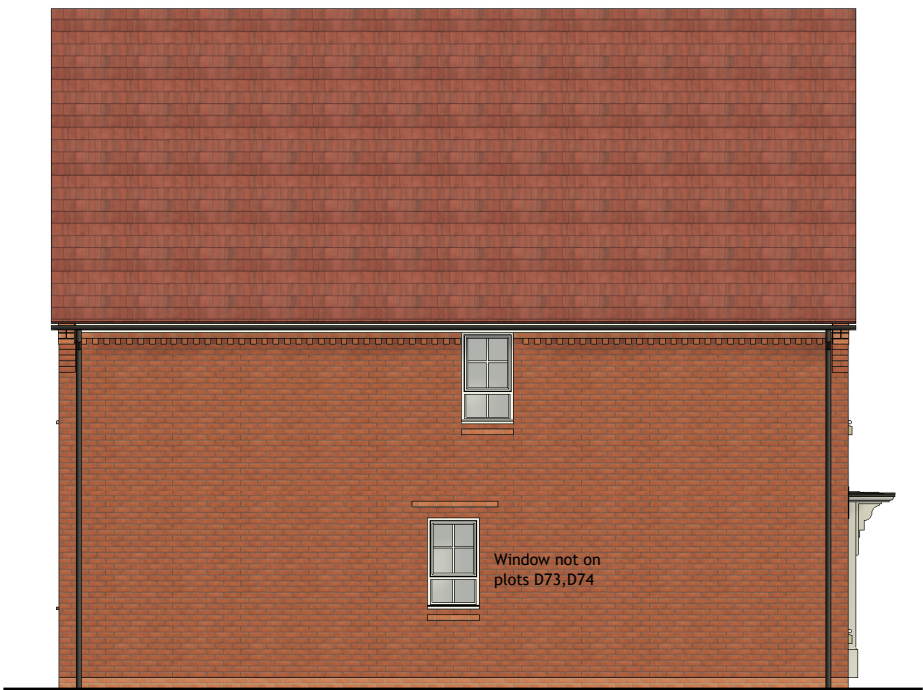
Left Elevation
