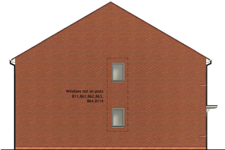
Left Elevation
