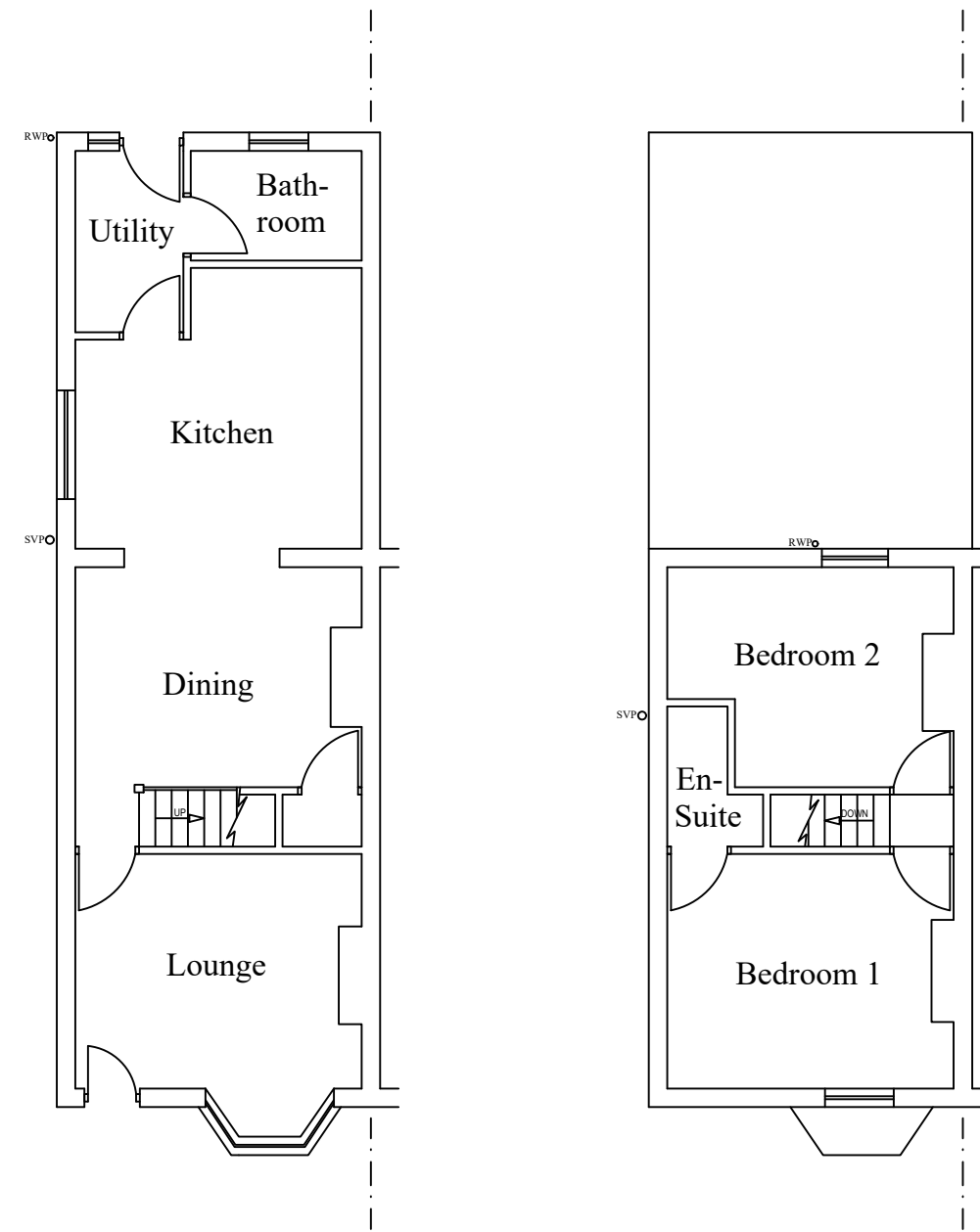
EXISTING GROUND FLOOR LAYOUT EXISTING FIRST FLOOR LAYOUT
