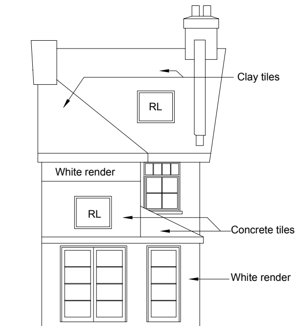
PRE-EXISTING REAR (NORTH) ELEVATION 1:100
