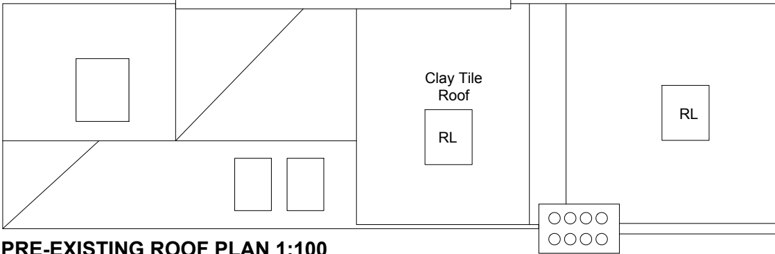
PRE-EXISTING ROOF PLAN 1:100
