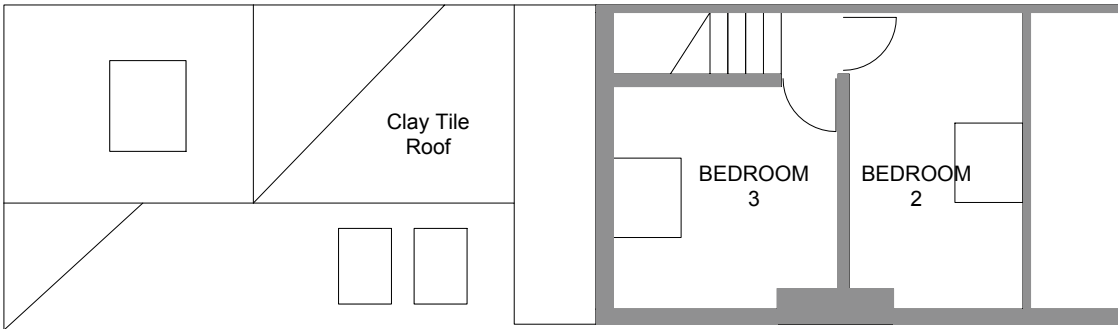
PRE-EXISTING ATTIC FLOOR PLAN 1:100
