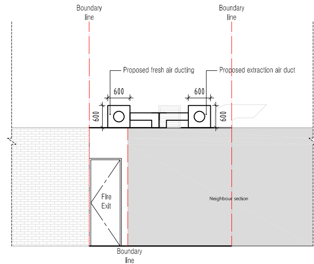
3 Proposed Rear Elevation Scale : 1 / 100 (A3)
