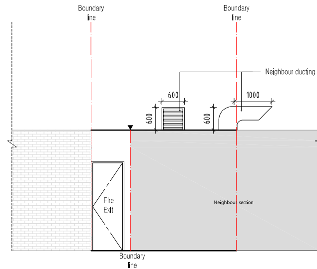
3 Existing Rear Elevation Scale : 1 / 100 (A3)
