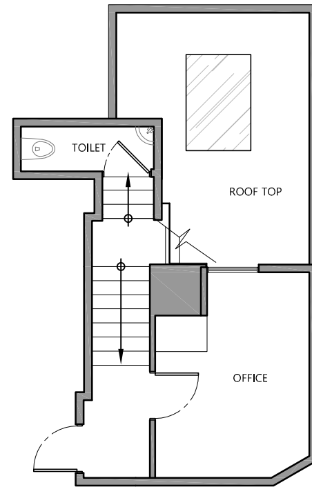
2 Existing First Floor Plan Scale : 1 / 100 (A3)
