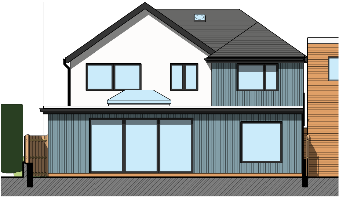
Proposed NorthEast Elevation 1 : 100
