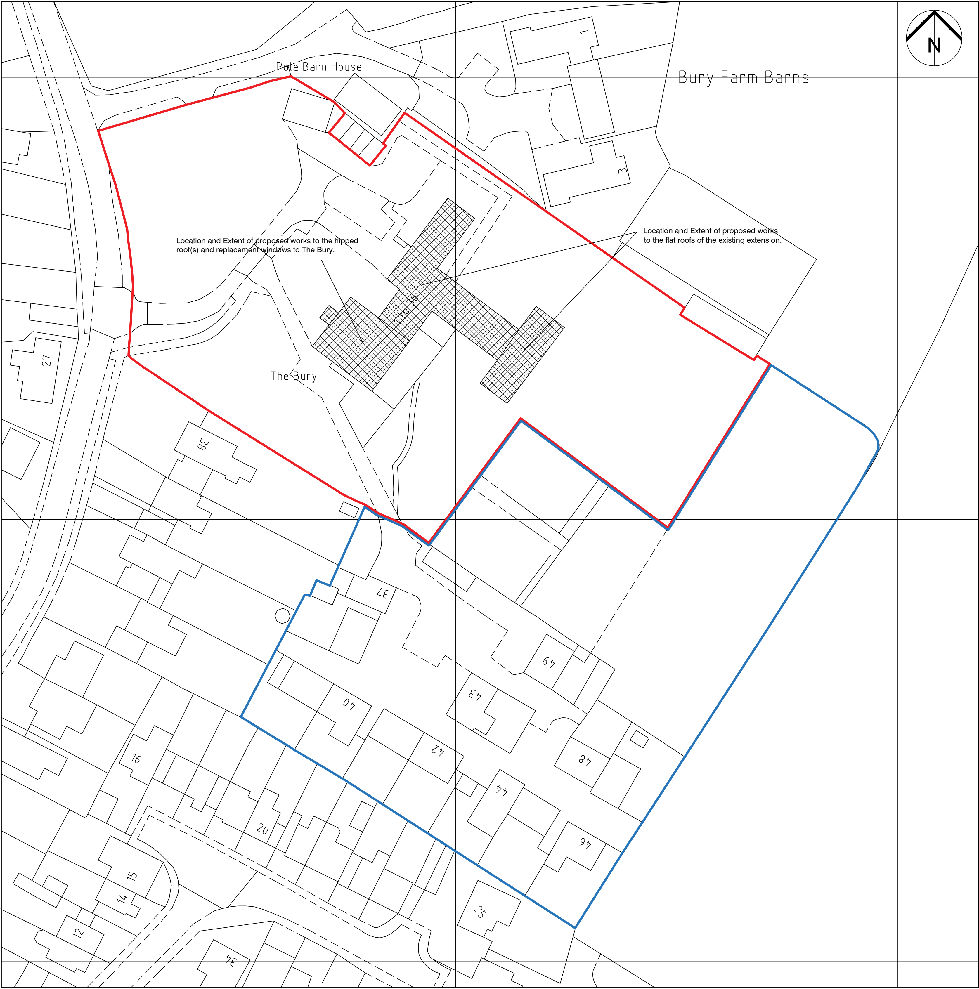
PROPOSED BLOCK PLAN (Scale 1:500)
