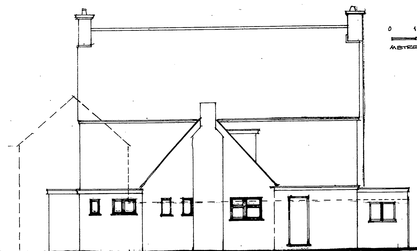
REAR ELEVATION
