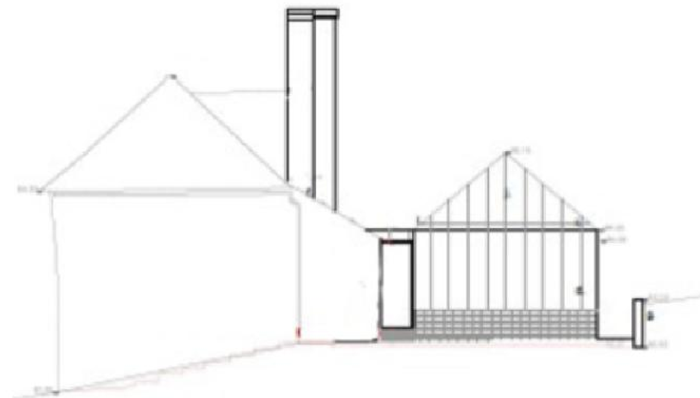
East Elevation
