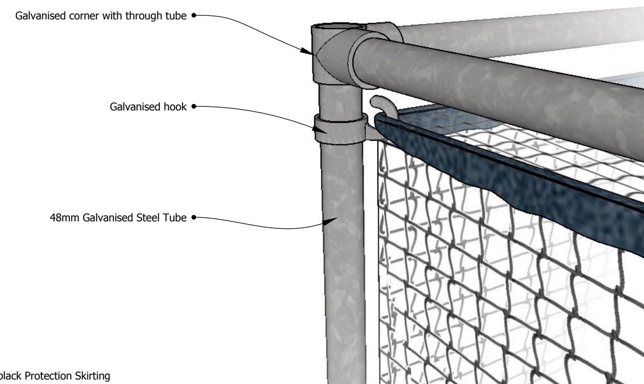
TOP CORNER DETAIL
