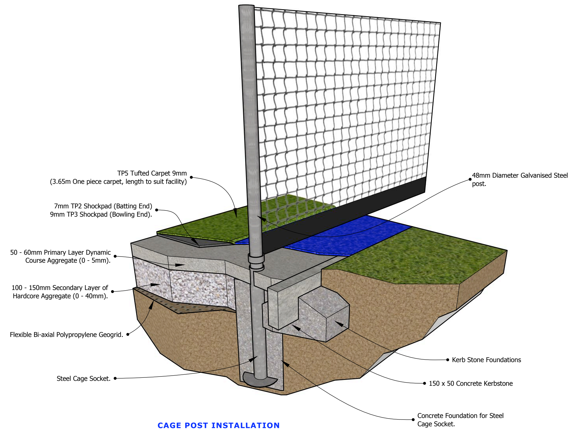
CAGE POST INSTALLATION
