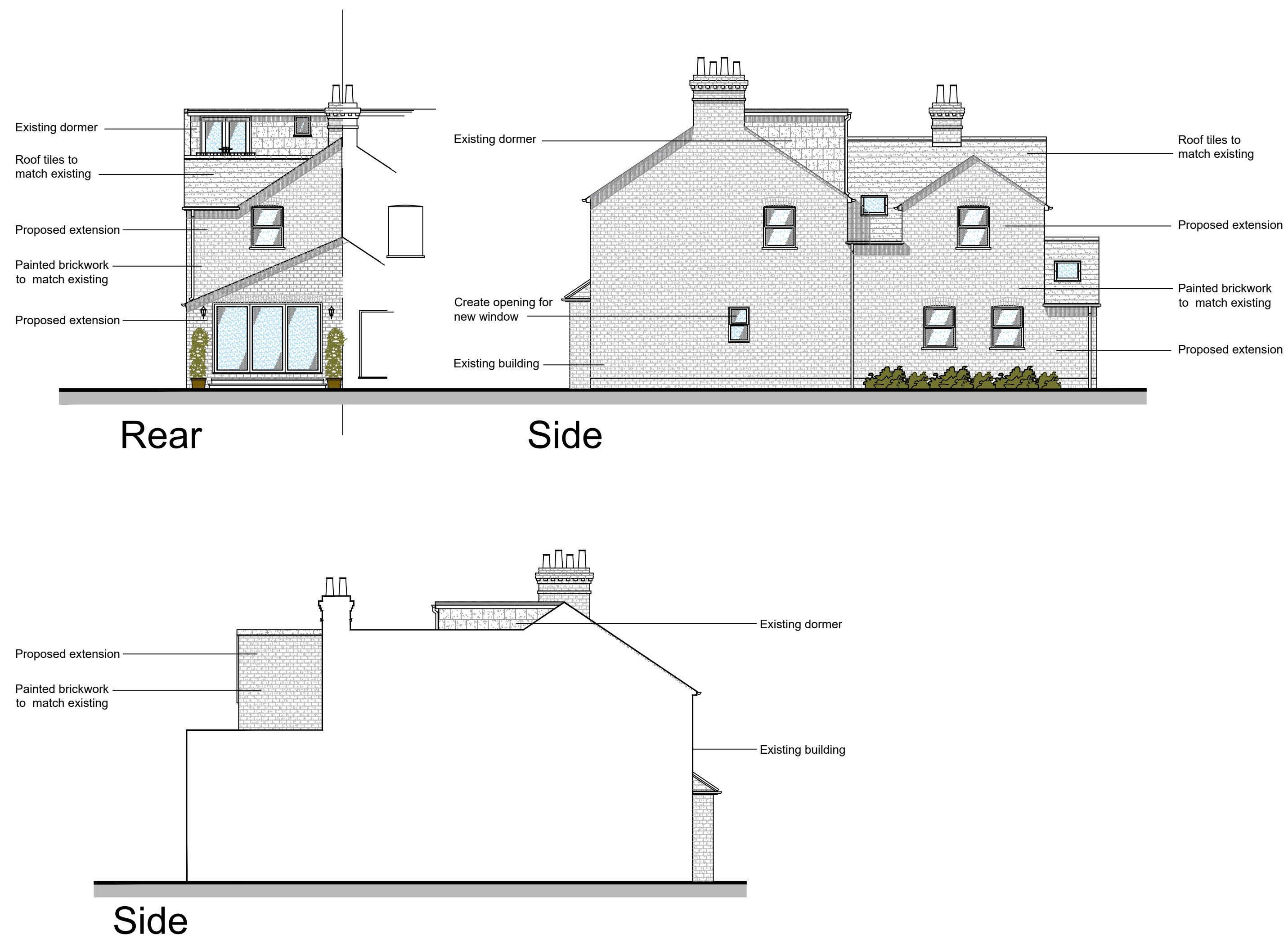
Proposed Elevations 1:100
