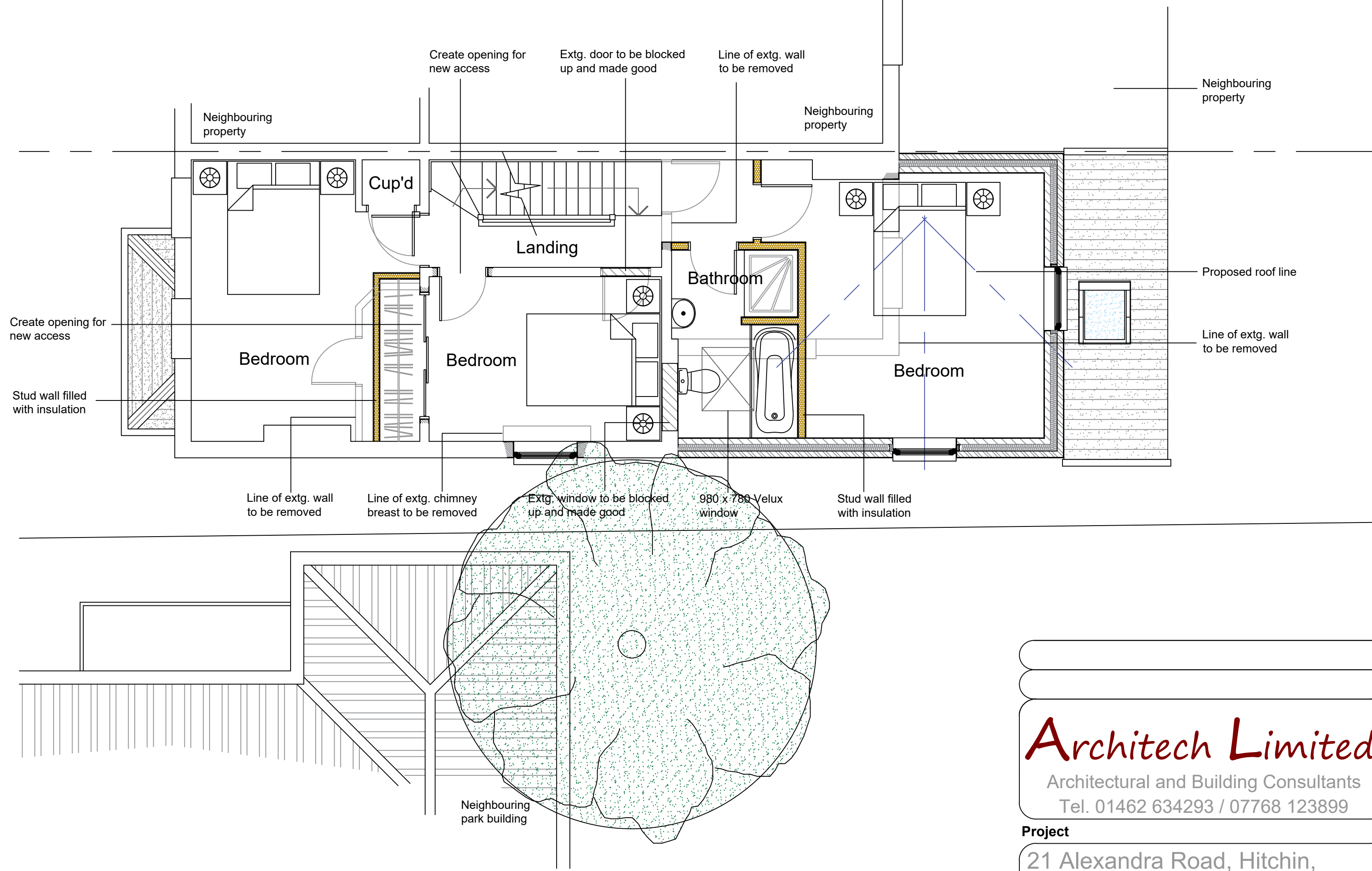
Proposed First Floor Plan 1:50
