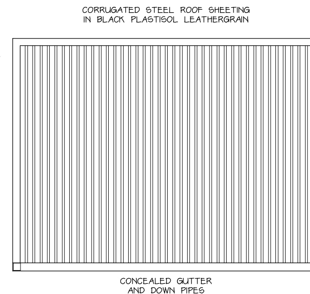
ROOF PLAN 1:50
