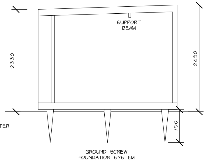
SECTION 1:50
