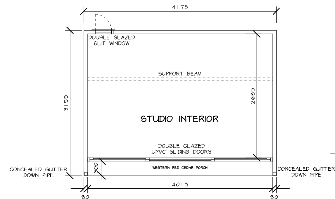
FLOOR PLAN 1:50
