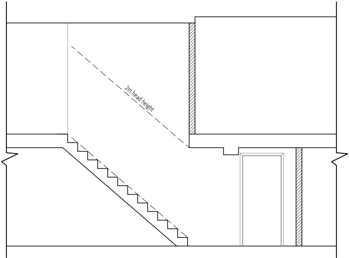
Stair Section @ 1/50
