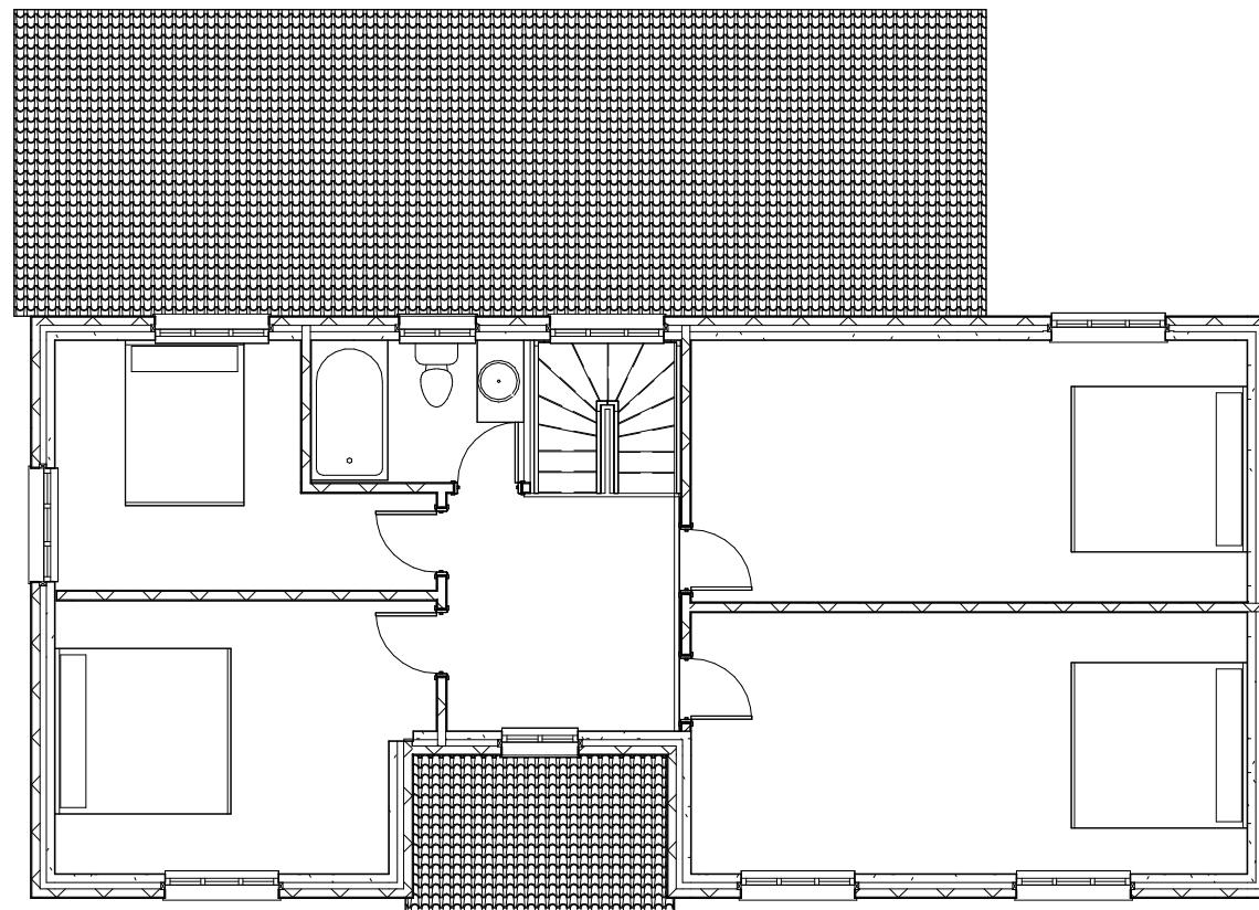
2 Proposed First Floor Plans 1 : 100
