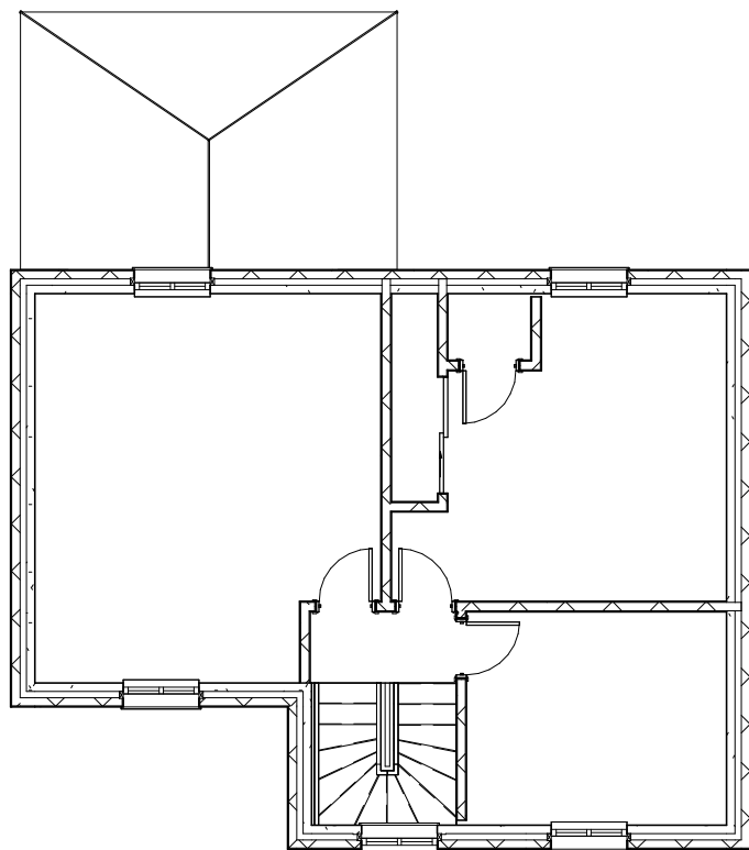
1 Existing First Floor Plans 1 : 100
