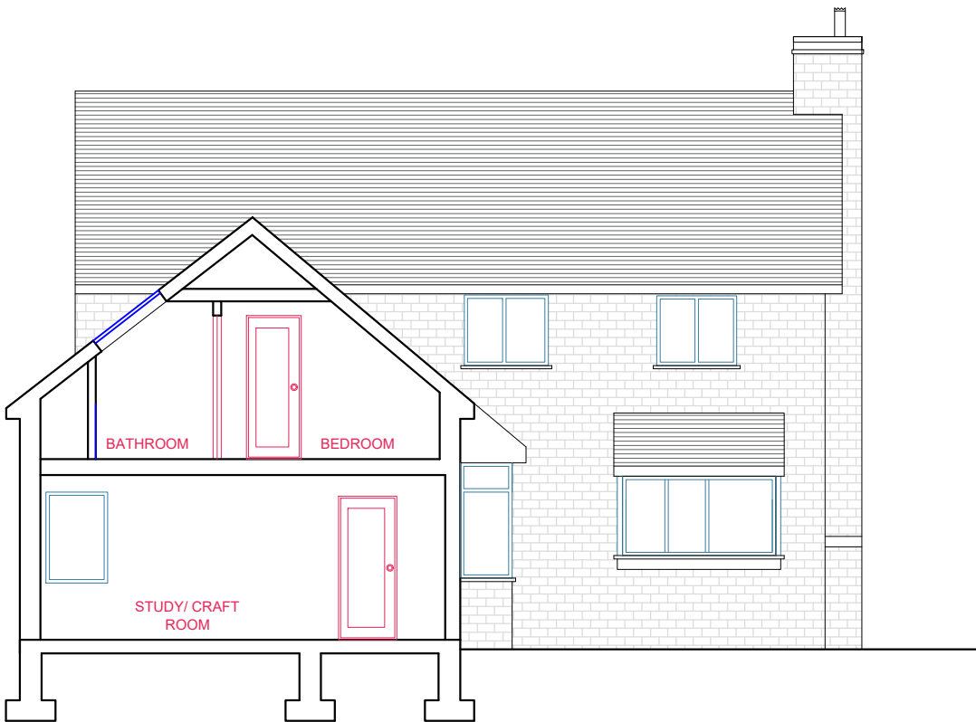
PROPOSED SECTION E-E
