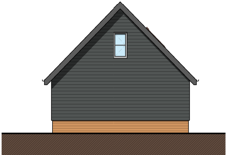
Proposed South Elevation 1 : 100
