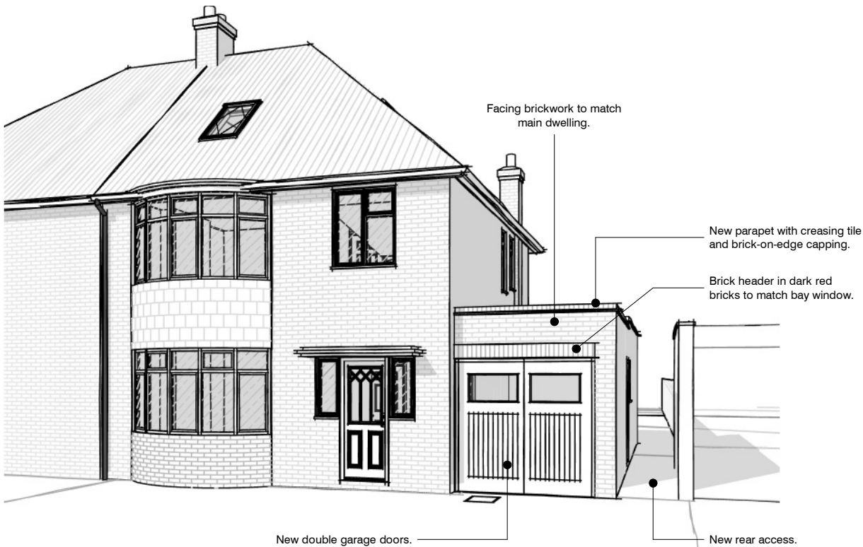
4 Front View - Proposed @A3
