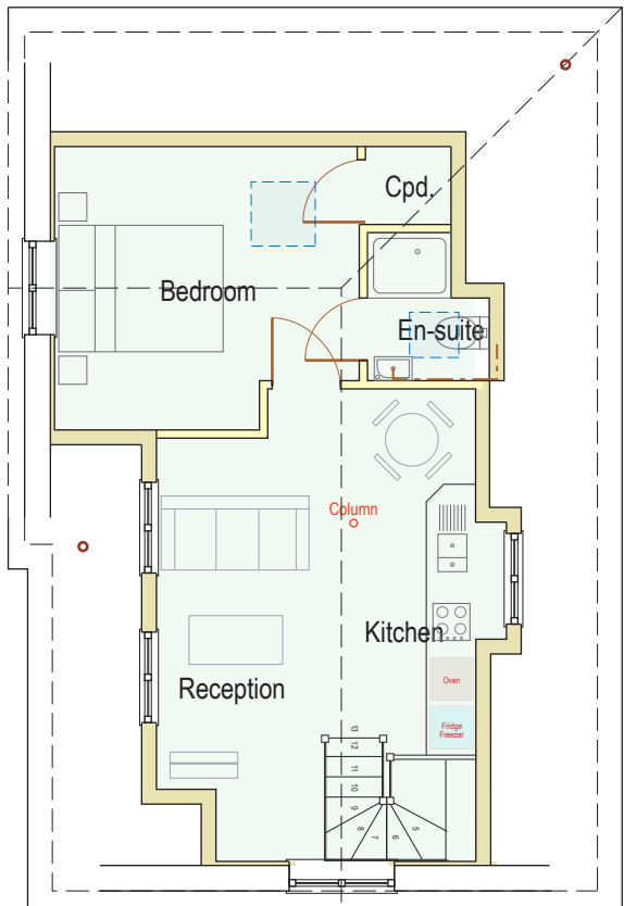
First Floor Plan (00m2)
