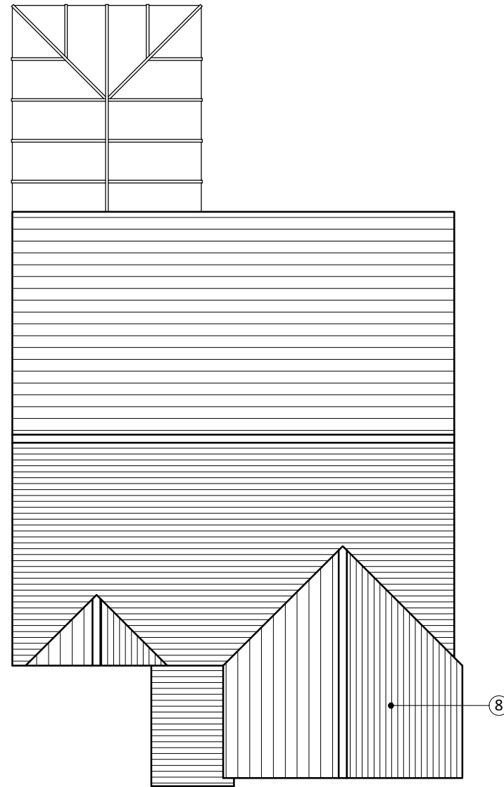
ROOF PLAN
