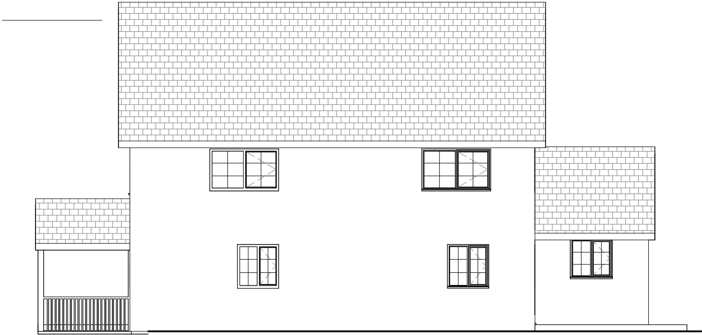
Rear Elevation 1 : 100
