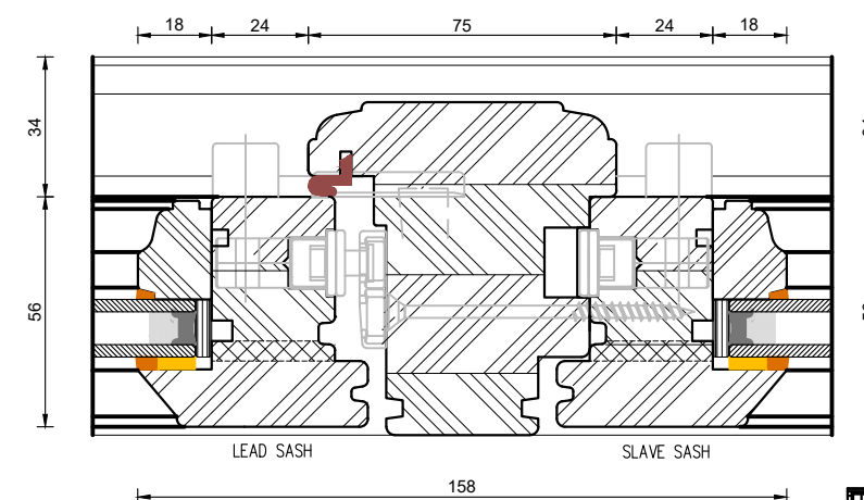
Heritage Slim-Line Flush Casement Window Flying Mullion (Lead / Slave Sash)
