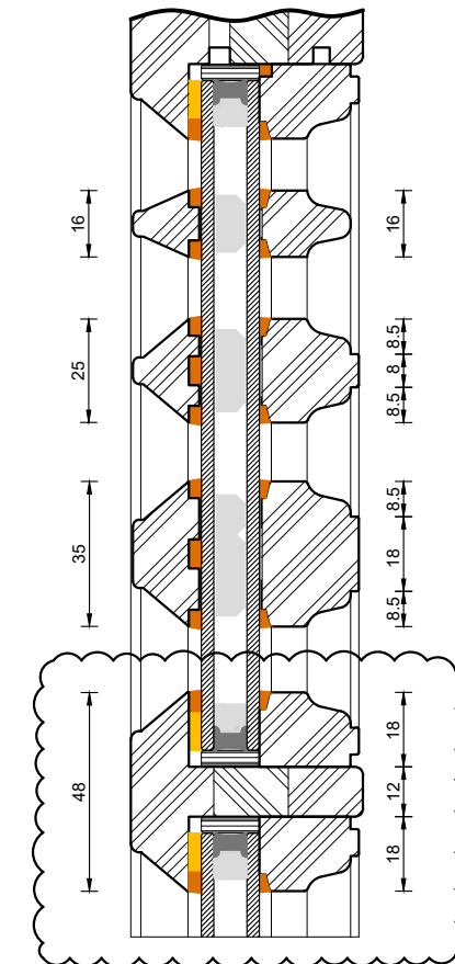
Heritage Slim-Line Flush Casement Window Bar Options
