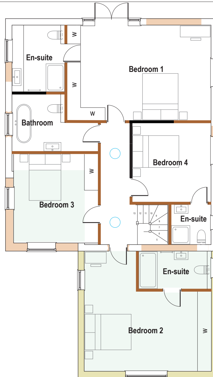
First Floor Plan (30.4m2)
