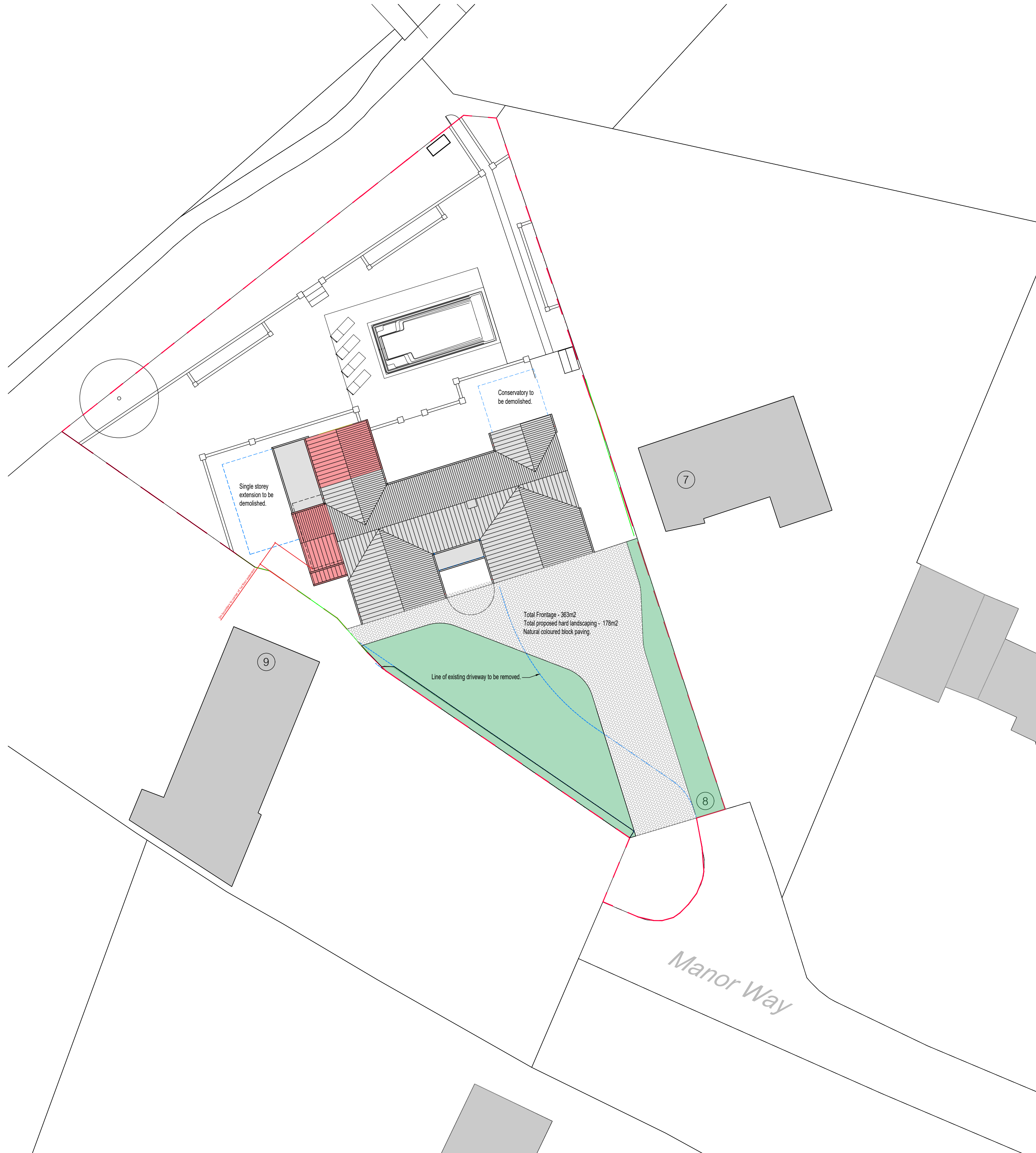
PROPOSED BLOCK PLAN AT 1 : 200
