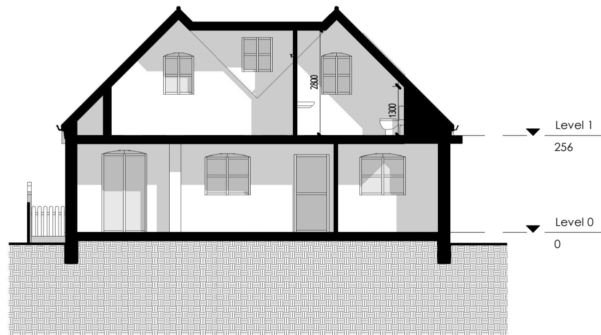
Proposed Cross Section 1:100
