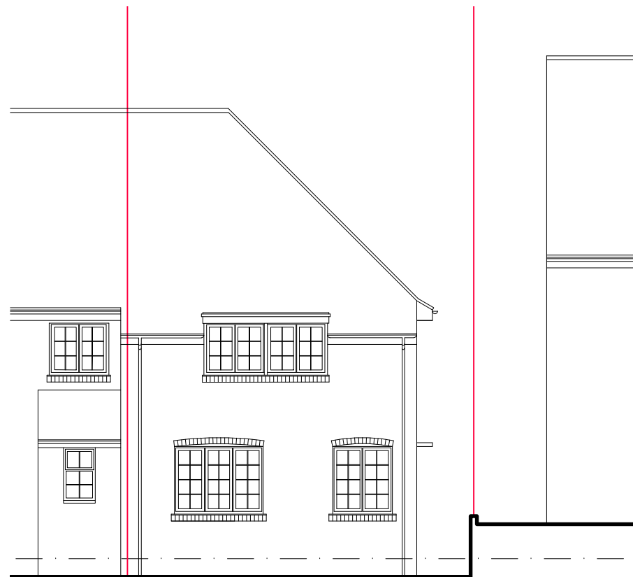
FRONT ELEVATION – EXISTING (1:100)
