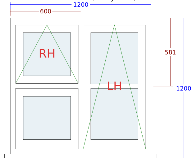
5. Flush Casement Window (Utility Rear.)
