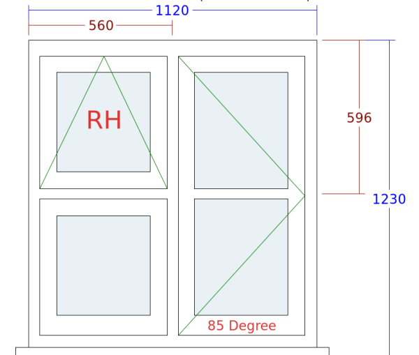
6. Flush Casement Window (W.C. Rear.)
