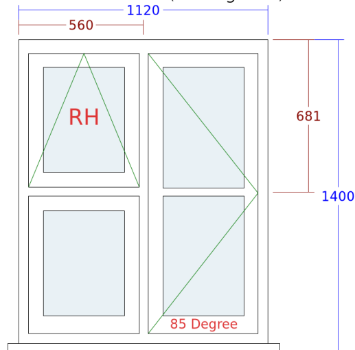
5. Flush Casement Window (Utility Rear.)
