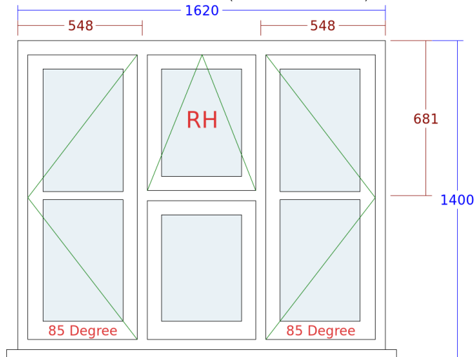
4. Flush Casement Window (Utility Rear.)
