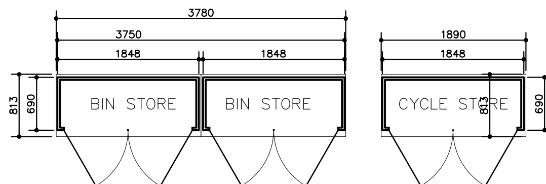
CYCLE STORE PLAN
