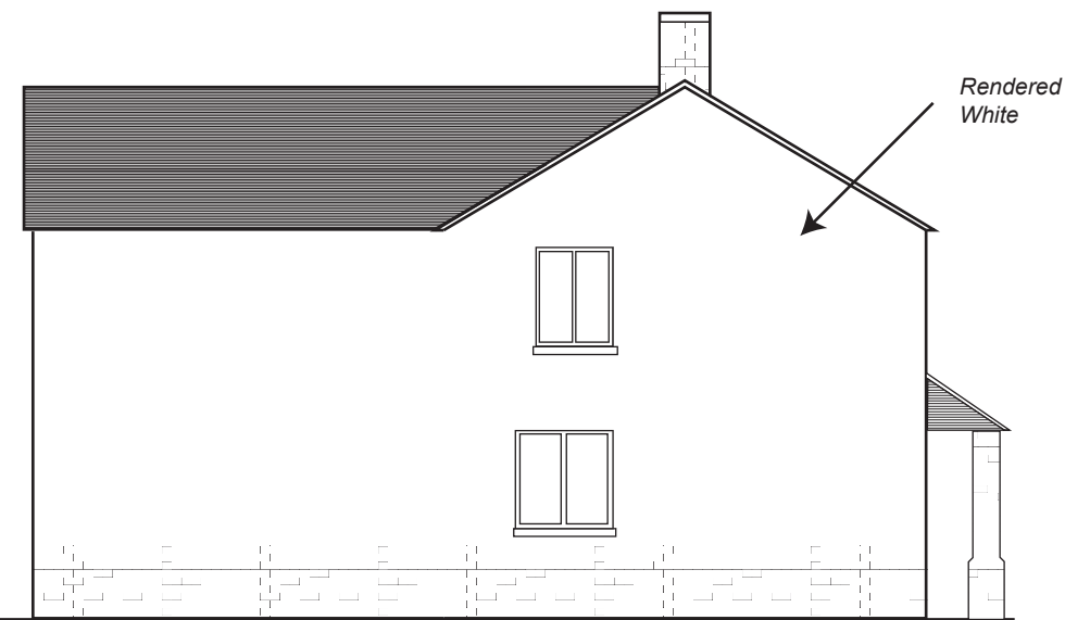
Side (South East) Elevation Scale 1:100
