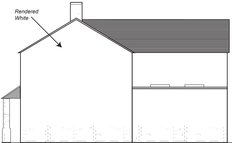
Side (North West) Elevation Scale 1:100
