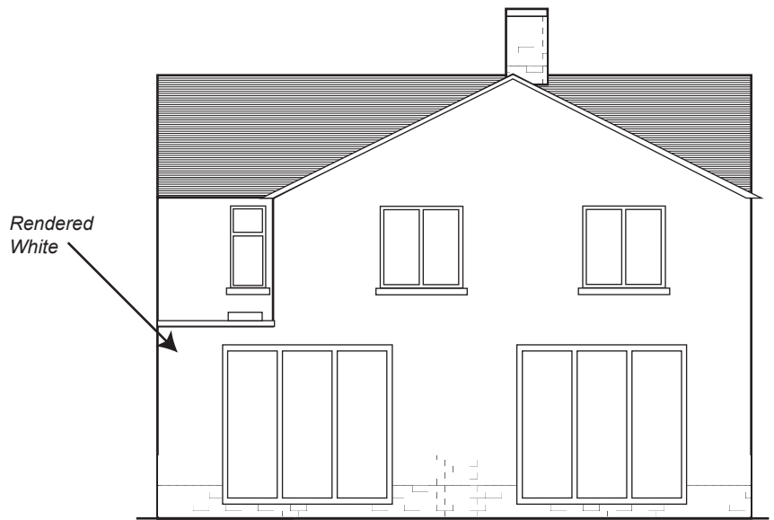
Rear (South West) Elevation Scale 1:100
