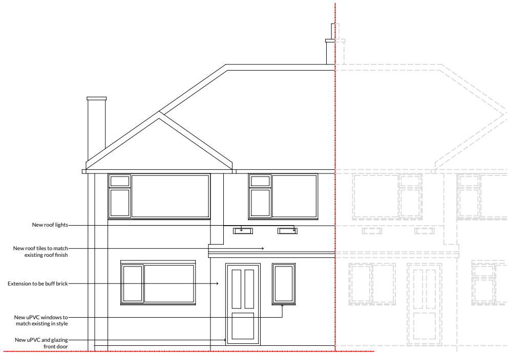
[01] PROPOSED ELEVATION 1 1:100
