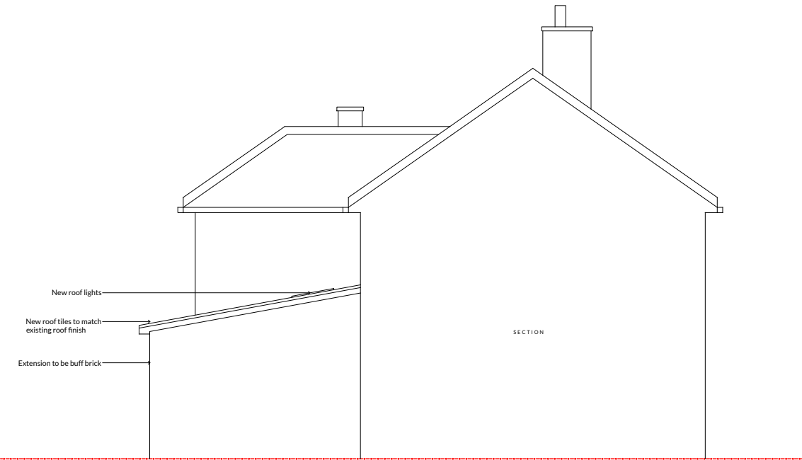
[03] PROPOSED ELEVATION 3 1:100
