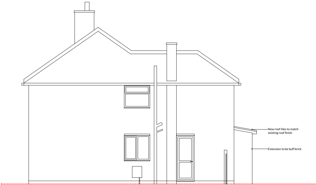
[02] PROPOSED ELEVATION 2 1:100
