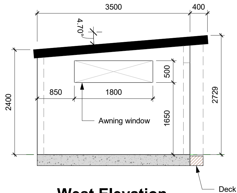
West Elevation
