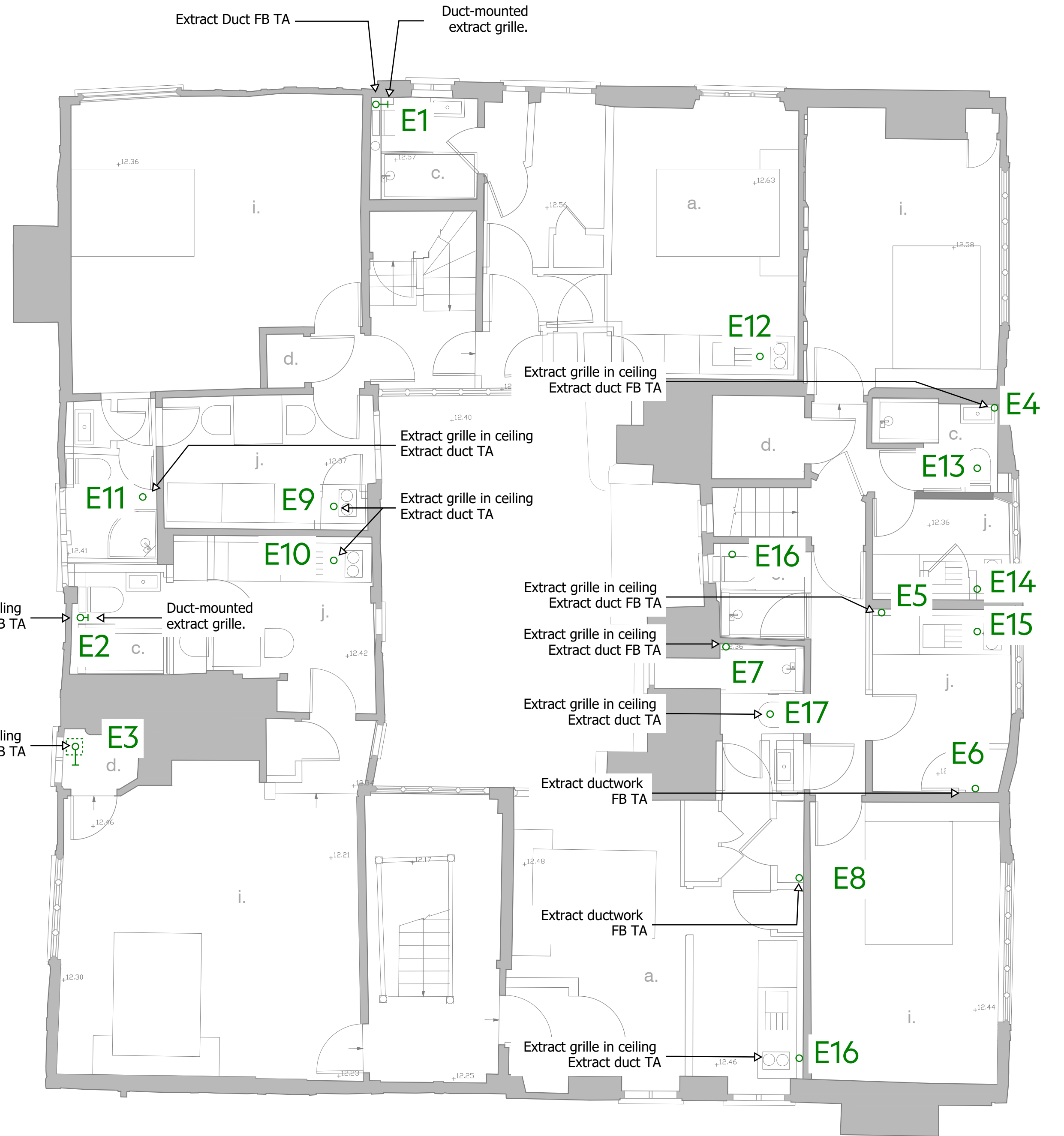
First Floor
