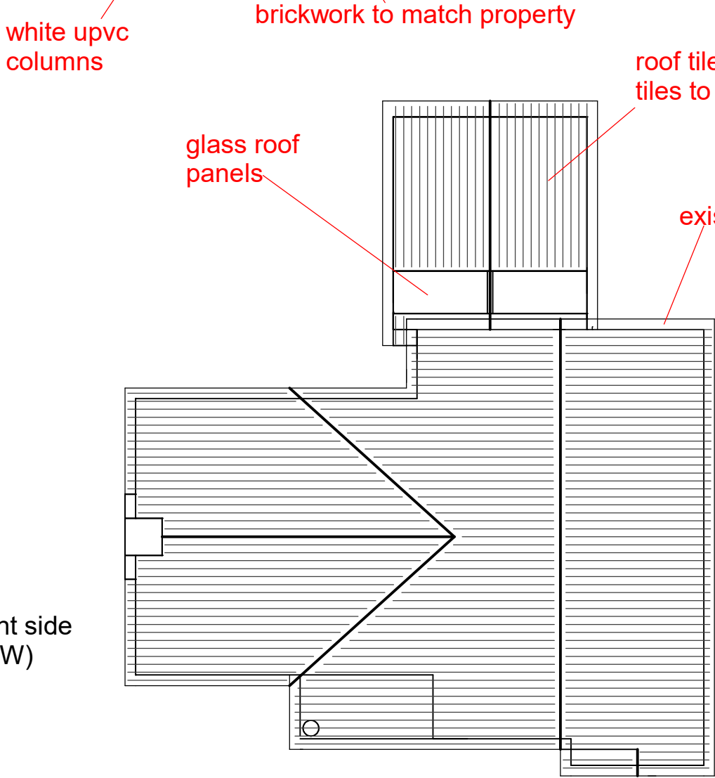
ROOF PLAN
