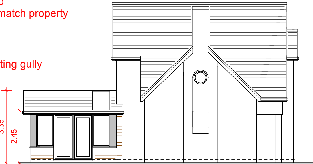
left side (northeast) elevation
