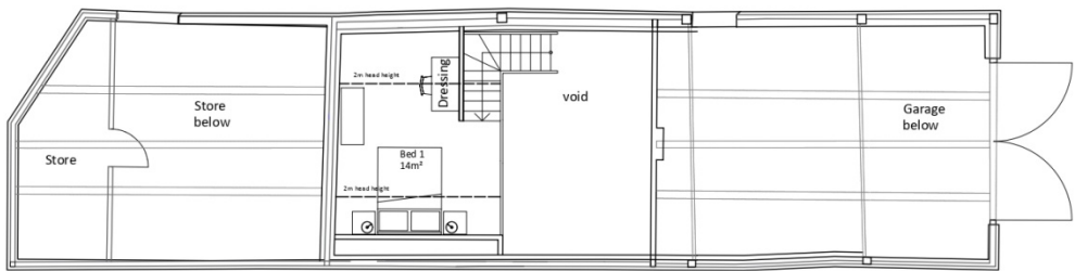
PROPOSED MEZZANINE FLOOR PLAN
