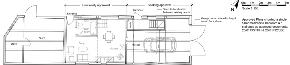
PROPOSED GROUND FLOOR PLAN 1:100
