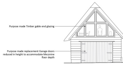
PROPOSED END ELEVATION
