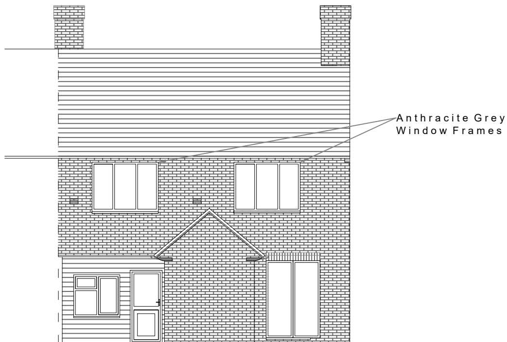
Rear Elevation
