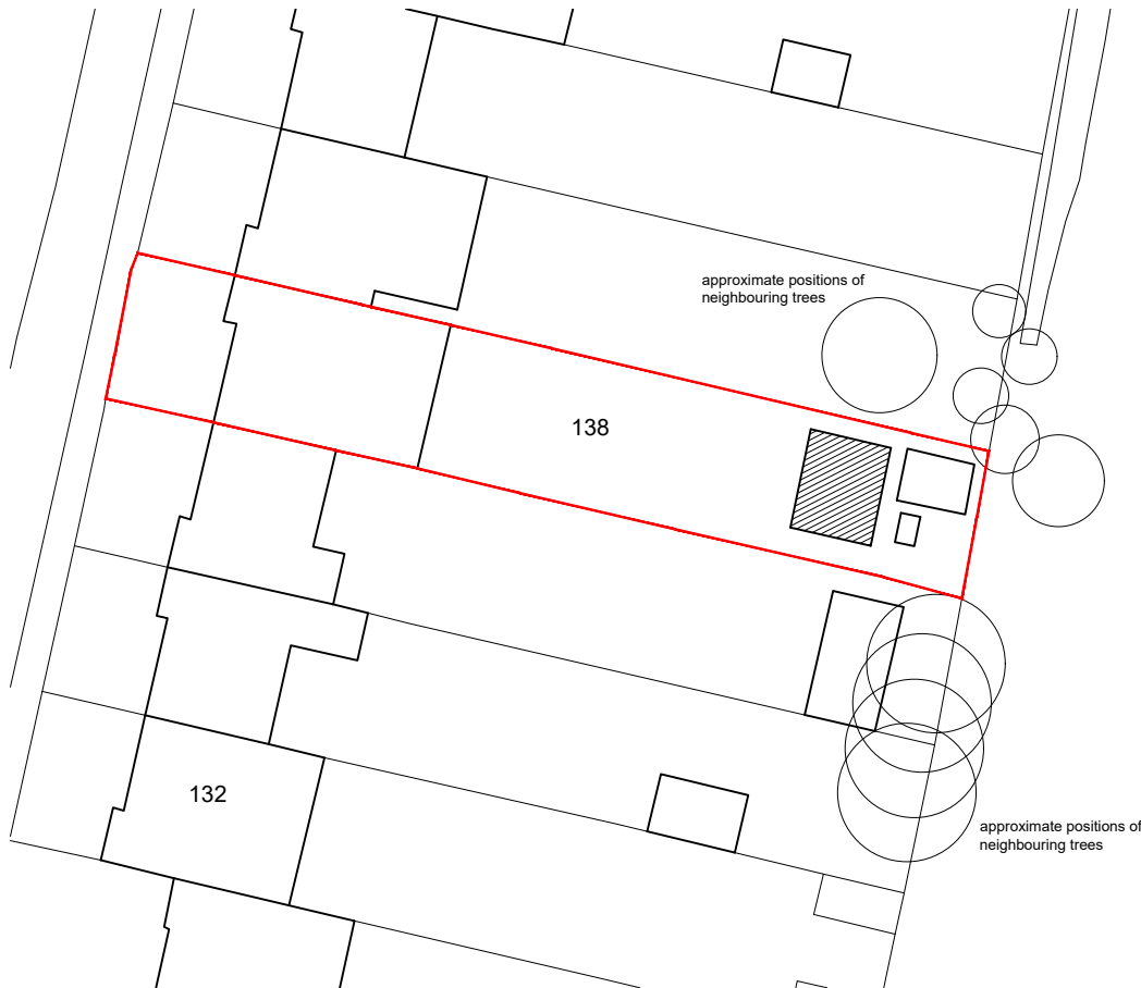
Block Plan 1:500
