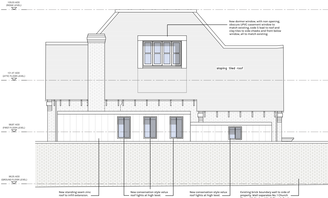
02 Proposed Side Elevation 1:100 @ A3
