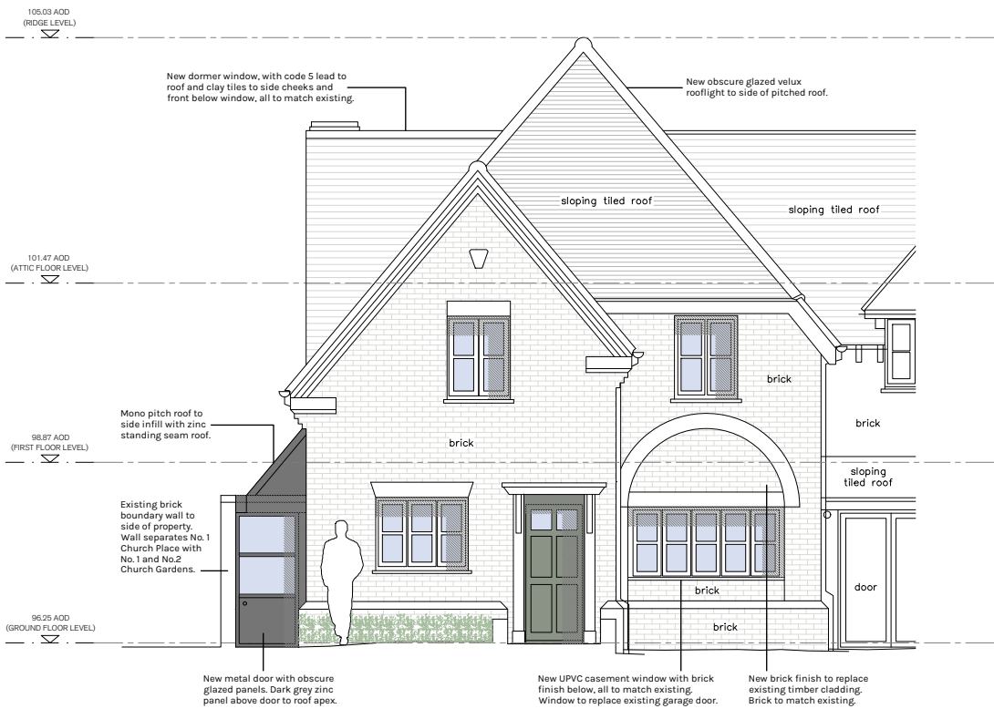
01 Proposed Front Elevation 1:100 @ A3
