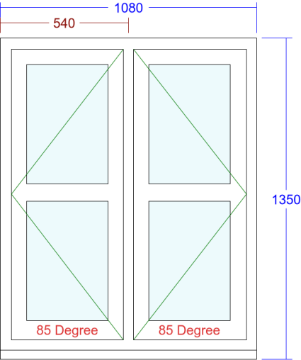
7. Flush Casement Window (Study Subject to survey)
