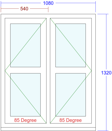
9. Flush Casement Window (Bedroom 2 Subject to survey)
