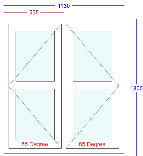
1. Flush Casement Window (Kitchen Subject to survey)
