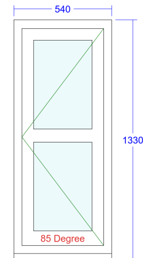
3. Flush Casement Window (Flag window to French Doors Subject to survey)
