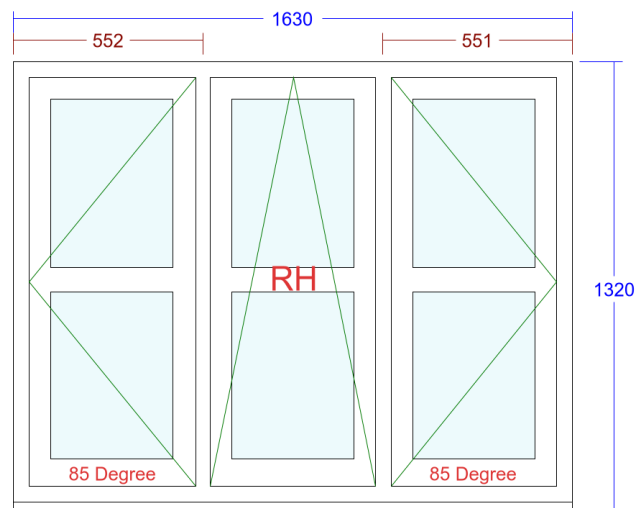
5. Flush Casement Window (Lounge Subject to survey)
