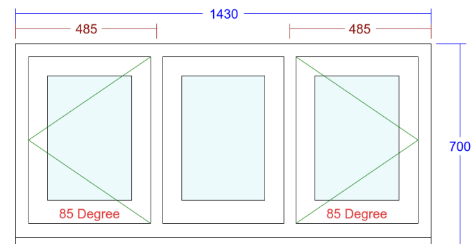
6. Flush Casement Window (Bathroom Subject to survey)
