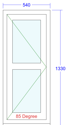
4. Flush Casement Window (Flag window to French Doors Subject to survey)
