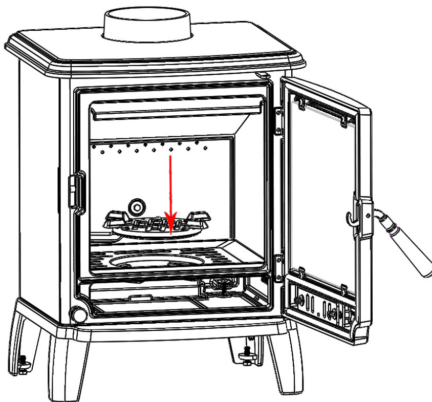
Fig 1.8 Riddling grate positioning. (As facing the stove) The riddling rod connecting hole in the riddling grate to be positioned to the left-hand side of the stove. The riddling rod is connected to the riddling grate eyelet hole to the left-hand side.
