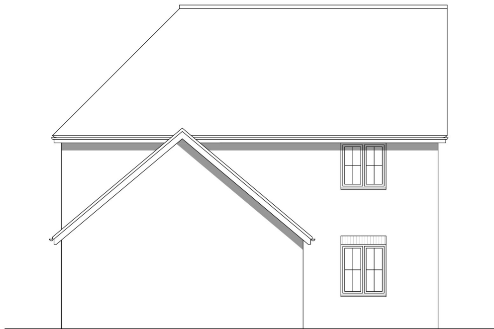
Rear Elevation
