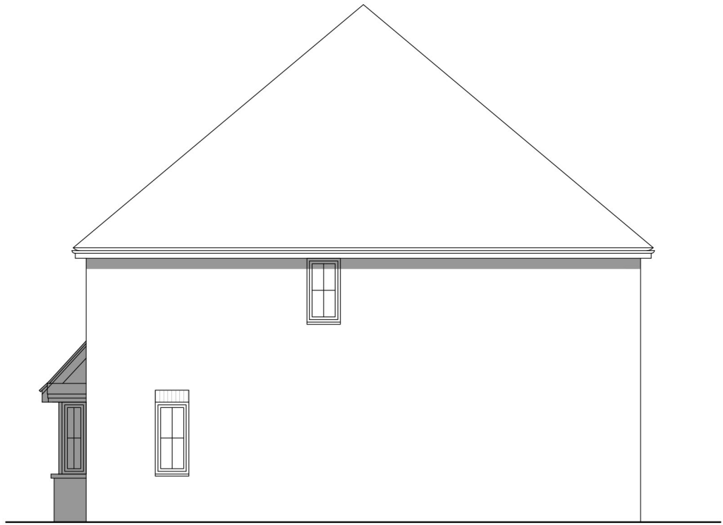
Side Elevation
