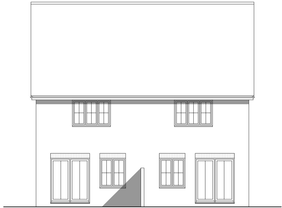
Rear Elevation
